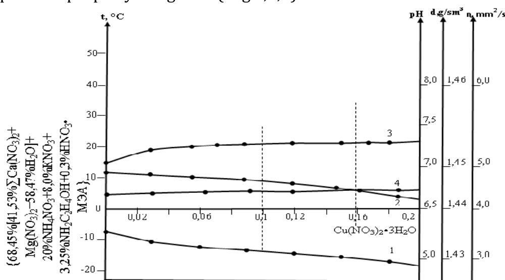
Fig.2. Dependence of changes in crystallization temperature (1), pH (2), density (3) and viscosity (4) of solutions on the composition in the system \{68.45\%[41.53\% \sum \text{Ca}(\text{NO}_3)_2 + \text{Mg}(\text{NO}_3)_2 + 58.47\% \text{H}_2\text{O}] + 20\% \text{NH}_4\text{NO}_3 + 8.0\% \text{KNO}_3 + 3.25\% \text{NH}_2\text{C}_2\text{H}_4\text{OH} + 0.3\% \text{HNO}_3 \cdot \text{MEA}\} - \text{Cu}(\text{NO}_3)_2 \cdot 3\text{H}_2\text{O}
