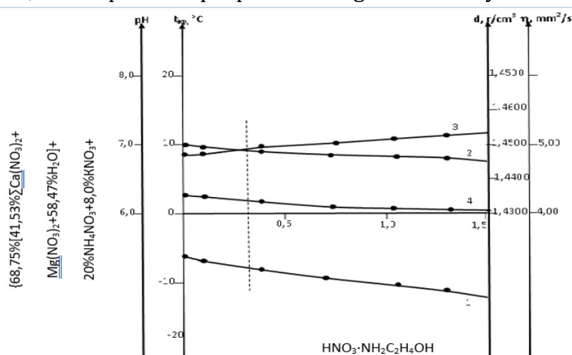
Fig.1. Dependence of changes in crystallization temperature (1), pH (2), density (3) and viscosity (4) of solutions on the composition in the system {68.75[41.53 % \Sigma Ca(NO 3 ) 2 + Mg(NO 3 ) 2 + 58.47 % H 2 O] +
