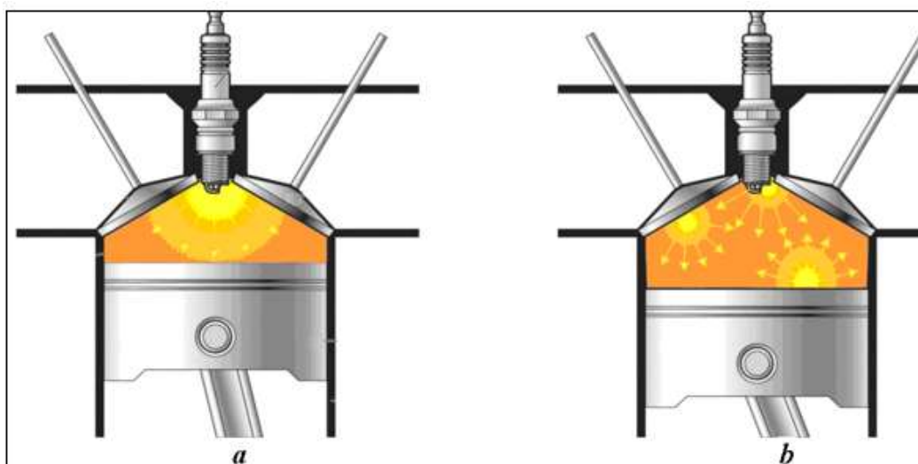
2-rasm. Benzinning yonish jarayoni
